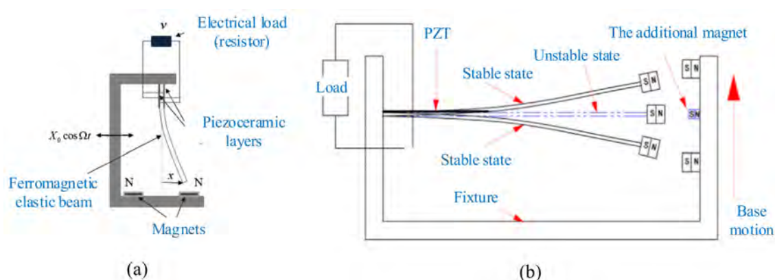
Figure 8. The bistable harvesters with magnetic attraction. (a) The piezomagnetoelastic energy harvester (reproduced with permission from [157]; published by Elsevier, 2010). (b) An improved bistable energy harvester (reproduced with permission from [158]; published by Elsevier, 2016).
