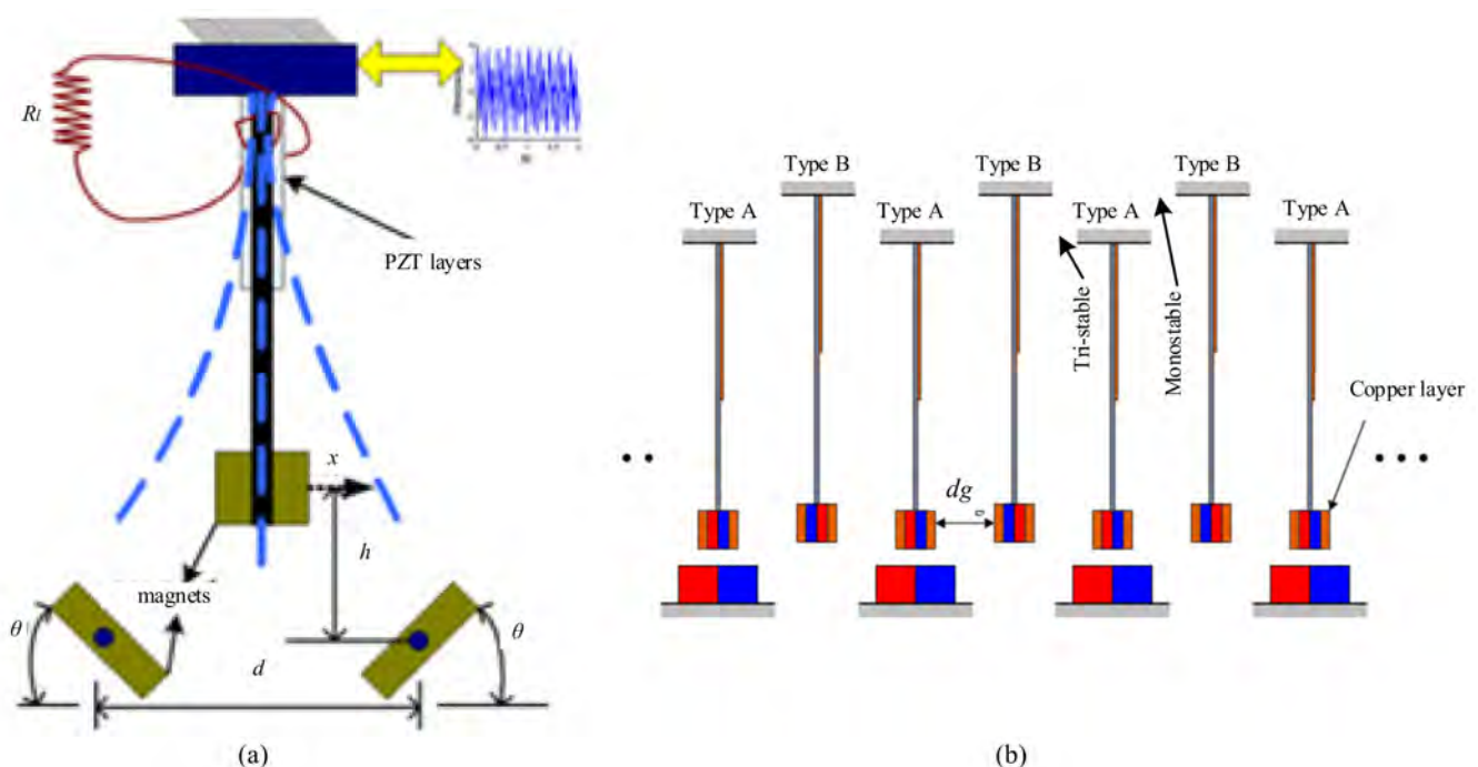
Figure 11. The tristable harvesters. (a) A tristable nonlinear oscillator (reproduced with permission from [161]; published by AIP, 2015). (b) A nonlinear multistable energy-harvester array (reproduced with permission from [165]; published by Elsevier, 2018).
