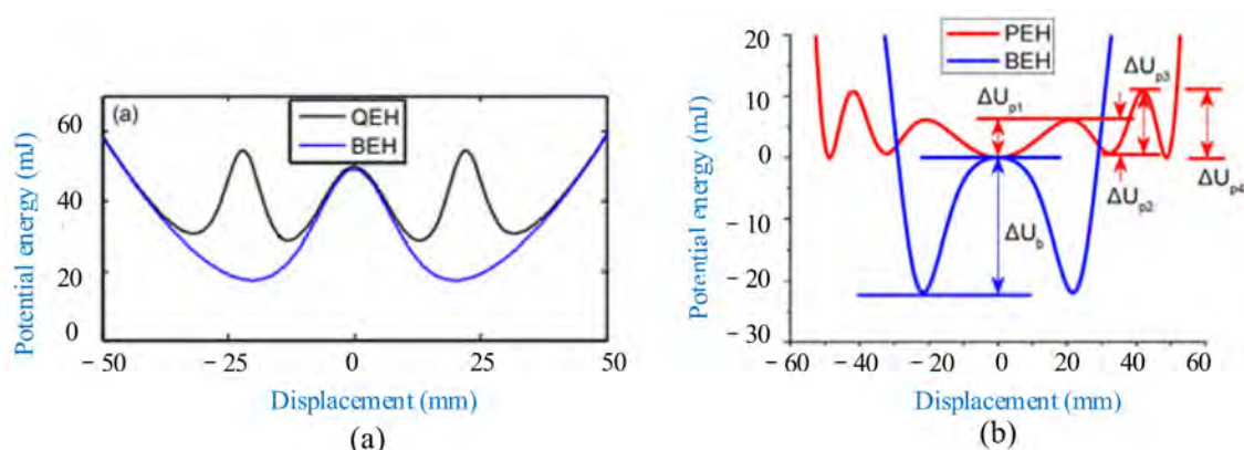
Figure 9. Potential energy shapes for: (a) Quadstable (QEH) and bistable (BEH) (reproduced with permission from [169]; published by Elsevier, 2016); and (b) pentastable (PEH) and bistable (BEH) (reproduced with permission from [174]; published by Elsevier B.V., 2017).
