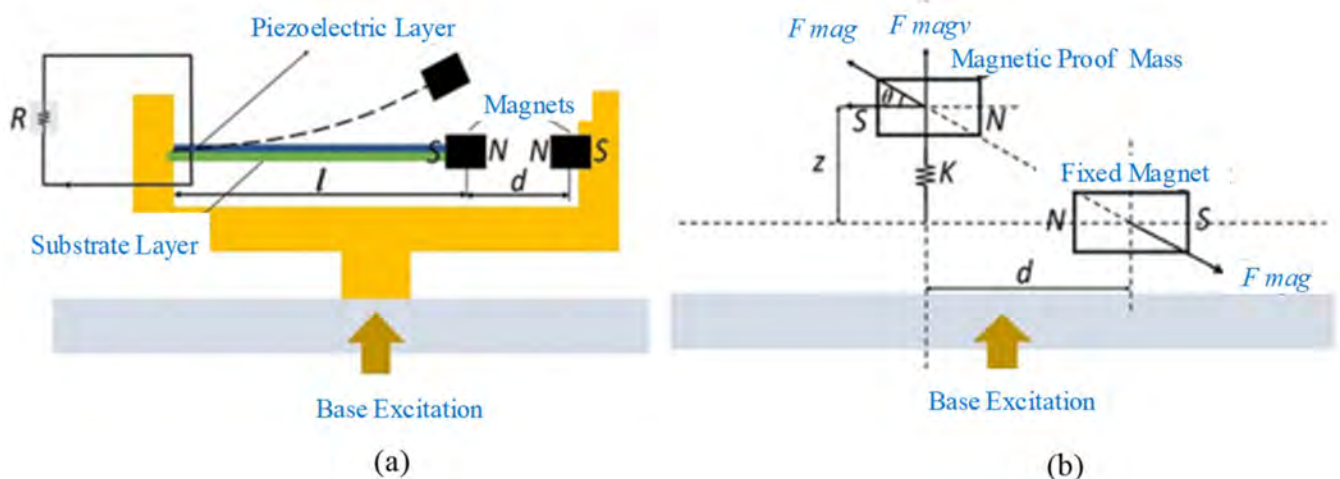
Figure 5. (a) Schematic of piezoelectric cantilever beam with magnetic proof mass (reproduced with permission from [136]; published by Wiley-VCH Verlag GmbH & Co. KGaA, Weinheim, 2015). (b) Free-body diagram of magnets (reproduced with permission from [136]; published by Wiley-VCH Verlag GmbH & Co. KGaA, Weinheim, 2015).
