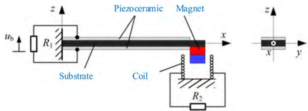
Figure 16. A typical hybrid energy harvester (reproduced with permission from [205]; published by MDPI, 2017).
