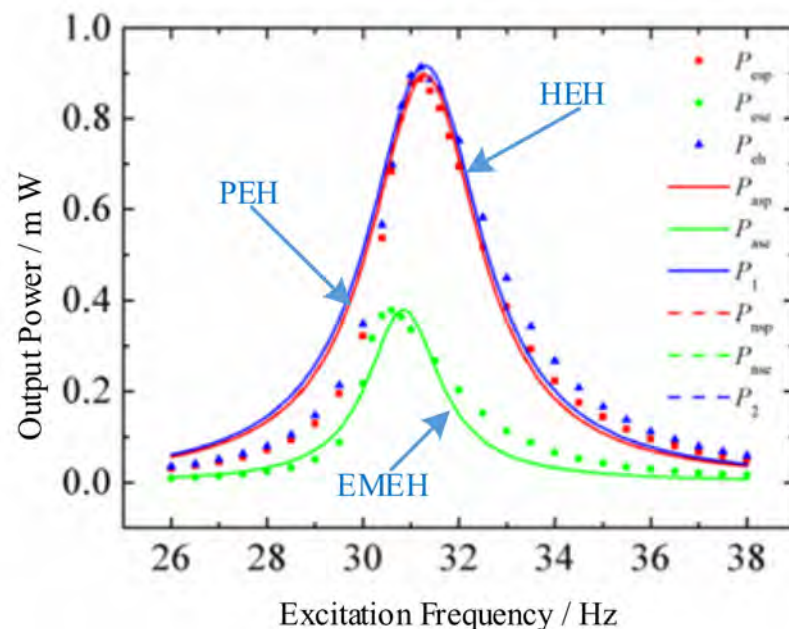
Figure 17. The optimal output power of the stand-alone piezoelectric energy harvester (PEH), stand-alone electromagnetic energy harvester (EME), and hybrid energy harvester (HEH) at different excitation frequencies (reproduced with permission from [205]; published by MDPI, 2017).
